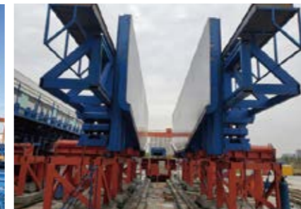
Prefabricated Bent Cap 预制盖梁
